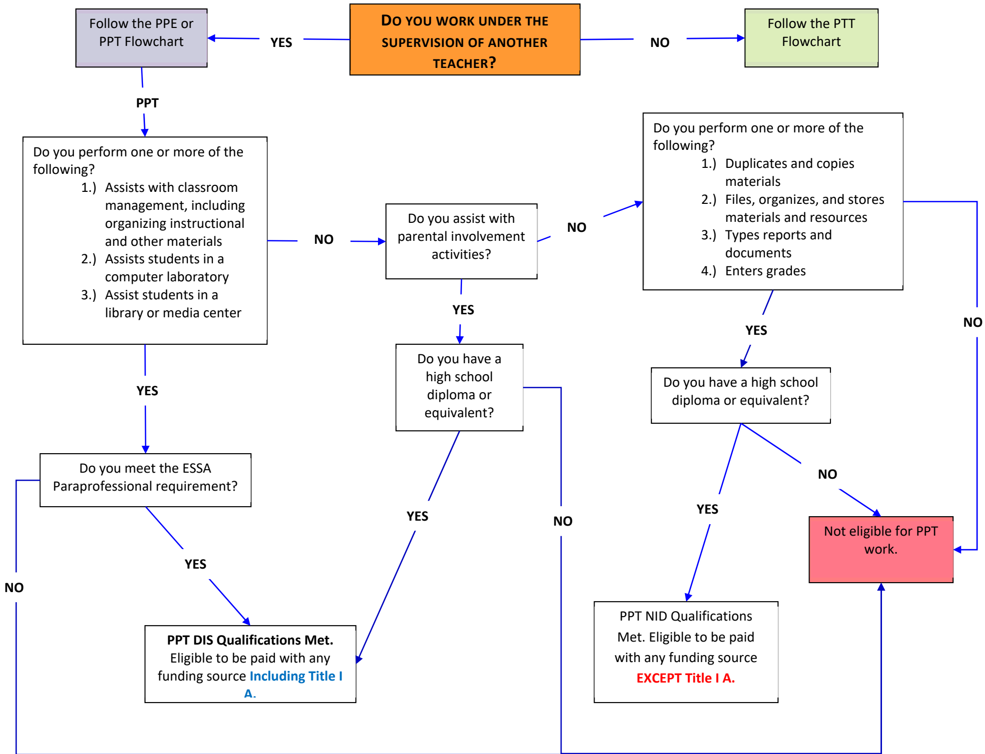
PPT FLOWCHART
